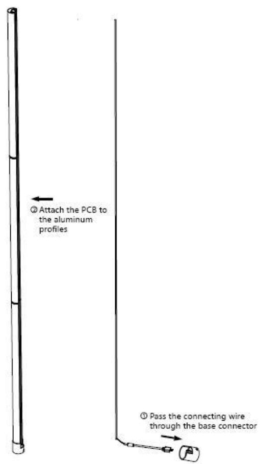
STEP2 Fixed lamp plate Pass the connecting wire through the base connector
